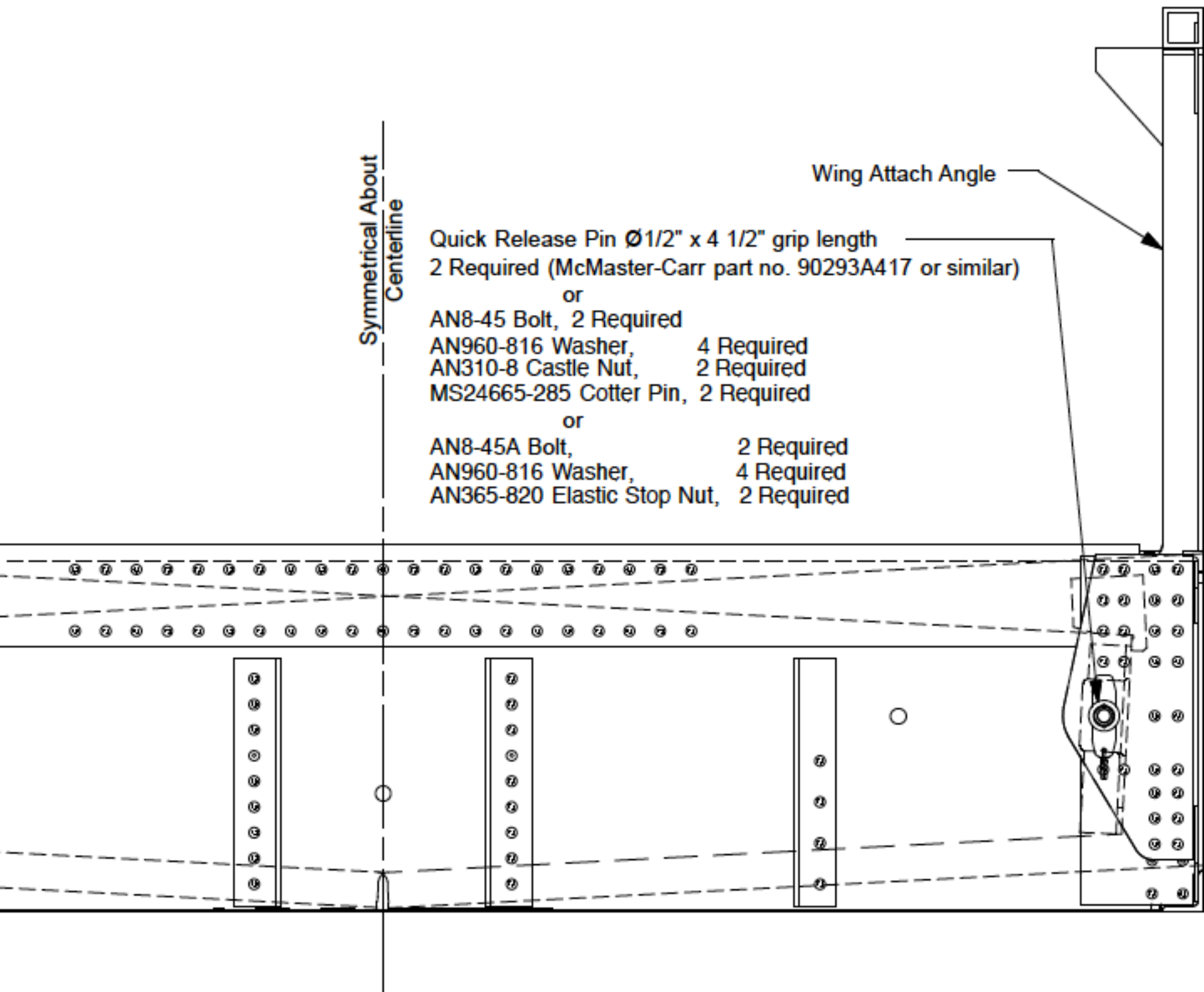
View A-A View Looking Forward at Main Spar Tunnel Scale: 1/4
