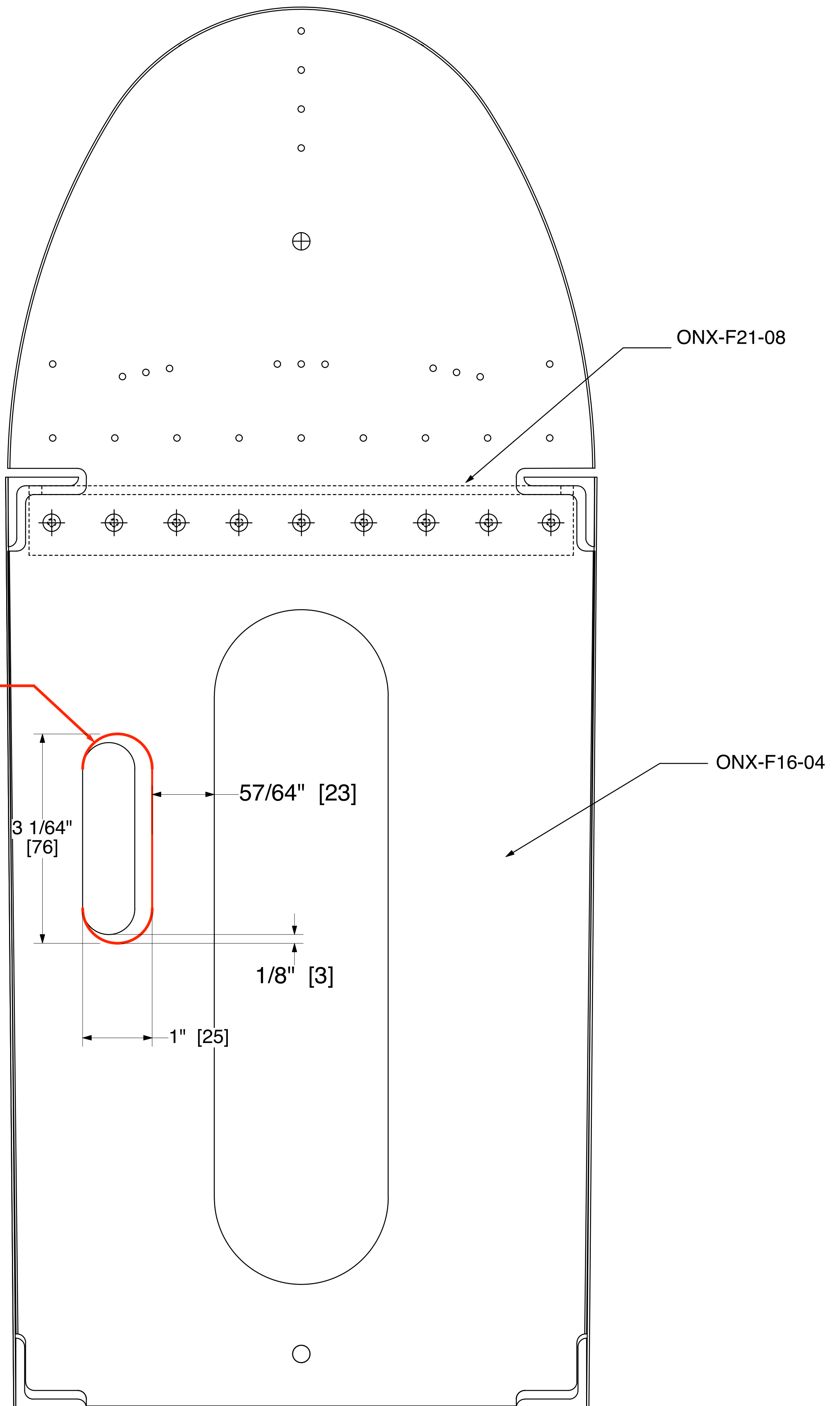
ONX-F17 Section D-D Bulkhead Position #4 Scale 1:4
